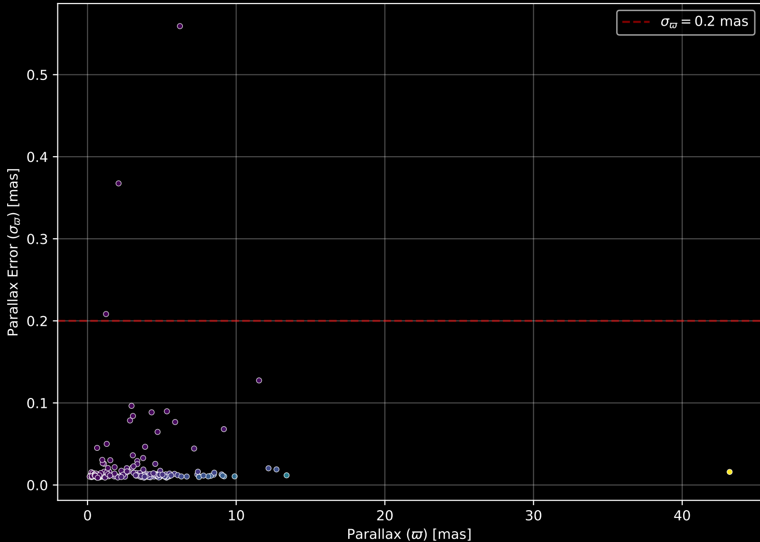
APOGEE DR17 Field: [CVZTILE_098+19_btx] Parallax Quality (n= 178)
