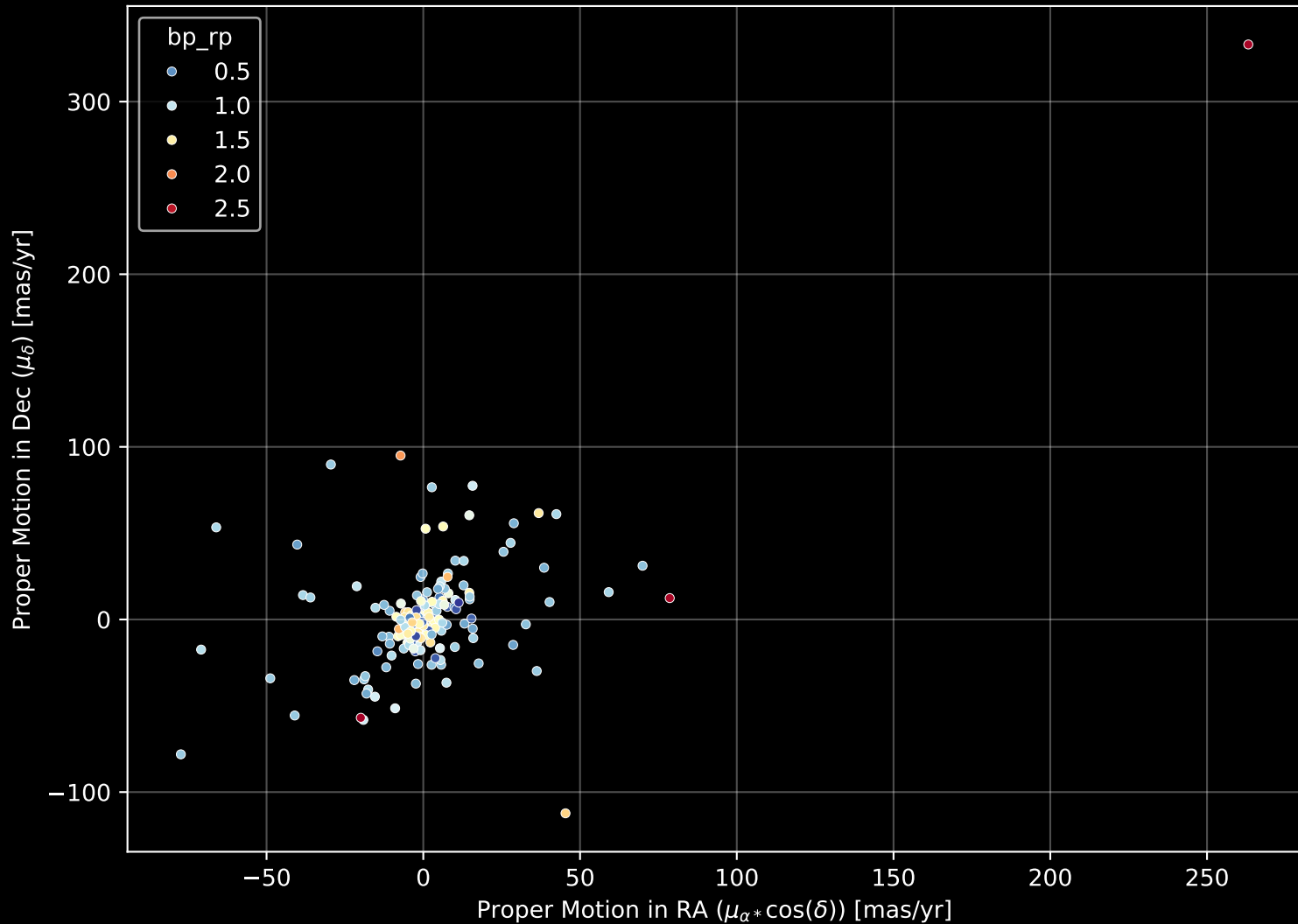
APOGEE DR17 Field: [CVZTILE_098+19_btx] Proper Motion Diagram (n= 178)
