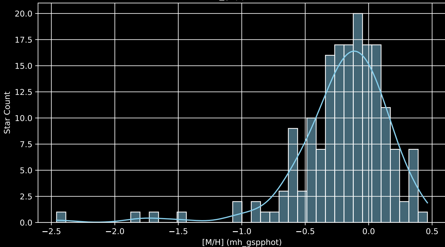
APOGEE DR17 Field: [CVZTILE_098+19_btx [M/H] (mh_gspphot) (n= 174)
