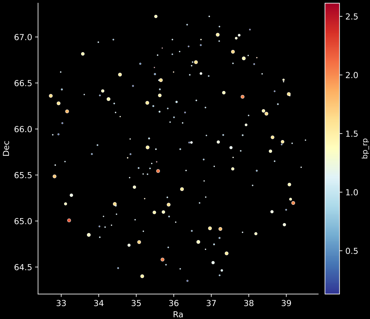
APOGEE DR17 Field: [CVZTILE_098+19_btx] Stars: 178
