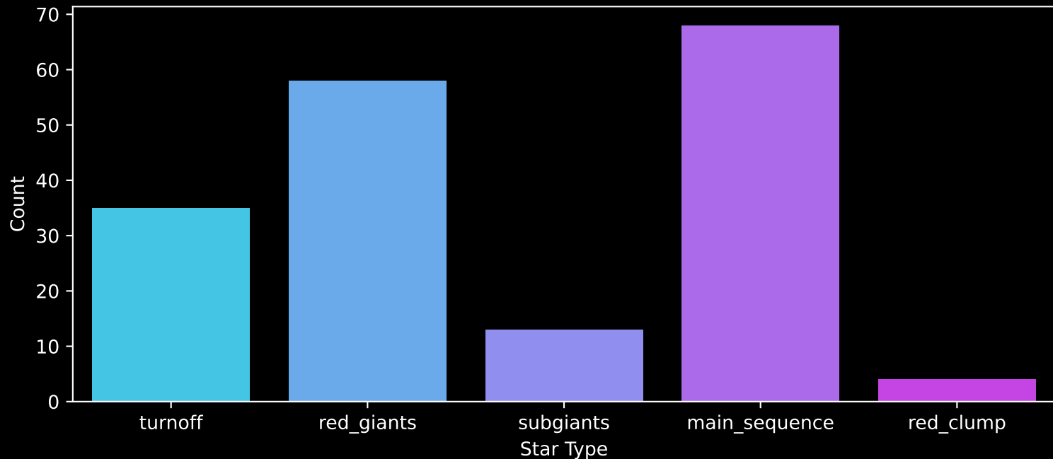
APOGEE DR17 Field: [CVZTILE_098+19_btx] Count plot of Star Type
