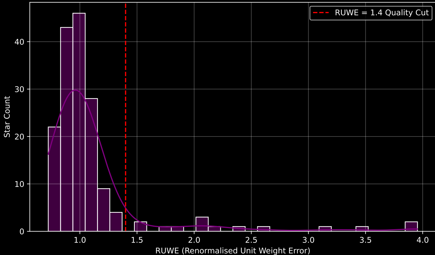
GAPOGEE DR17 Field [CVZTILE_098+19_btx] RUWE Distribution (n= 166)
